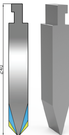
USH 240 B 86°60'30" R2,0
