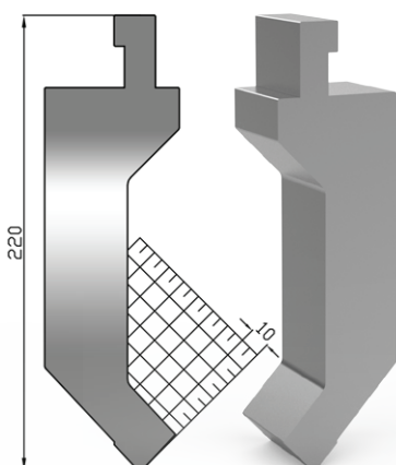
USH 220 A 86° R2,0
