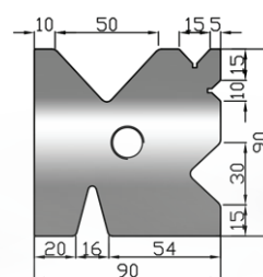
USH M 90 V10-15-30-50/86°+V16/30°
