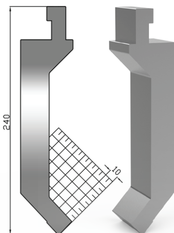
USH 240 A 86° R2,0
