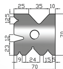
USH M 70 V9-12-15-24-35/86°+V12/30°
