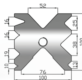
USH M100 V10-13-16-19-25-38-52-76/86°+V16/40°
